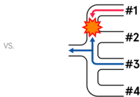
Exhaust interference in regular 4-1 exhaust manifold
