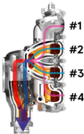
4-2-1 Performance Tuned Exhaust
